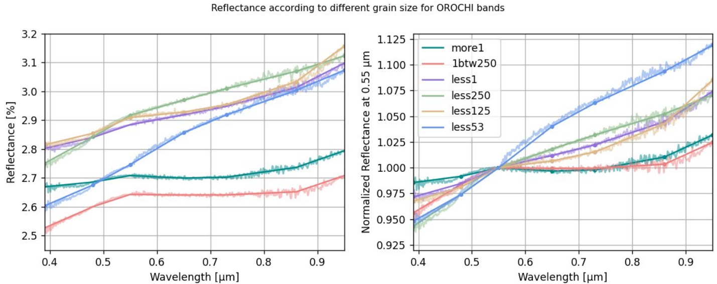
Figure 20 - OROCHI expected results according to its filter bands. (left) Reflectance spectrum (right) Normalized reflectance at 0.55\mu\text{m} . The letters represent the band given in Table 4. The blurry signals are the raw signals from UTPS-TB and the straight lines are the average values obtained in OROCHI conditions.
