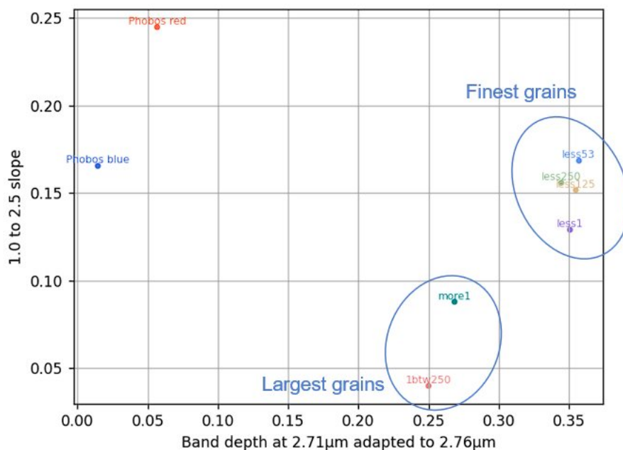
Figure 11 - Relationship between the slope from 1.0 to 2.5 \mu m and the band depth at 2.71 \mu m adapted to 2.76 \mu m.
