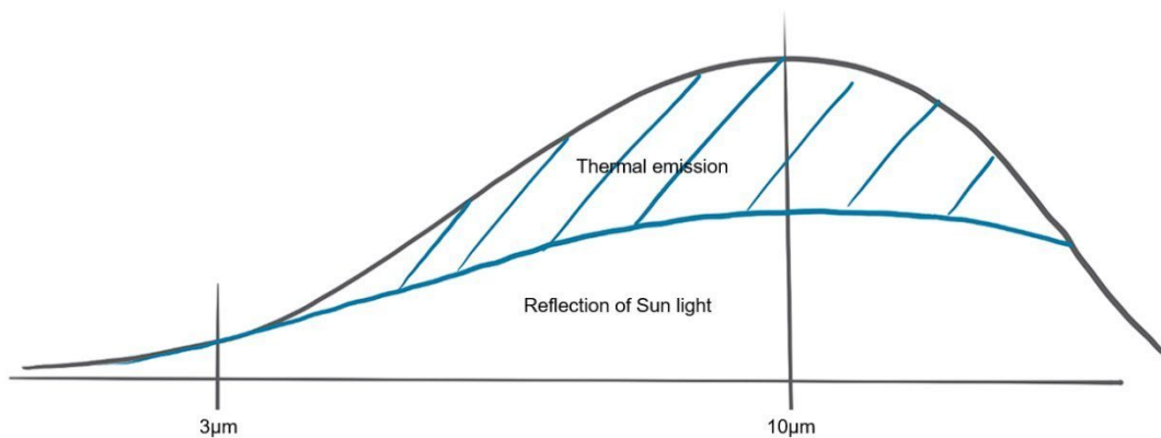
Figure 21 - Effect of thermal emission on reflectance spectra. The blue part corresponds to thermal emission effect, whereas the real reflectance is above that blue part. The 10\mu\text{m} range corresponds to the maximum value and 3\mu\text{m} is the location of MIRS study.
