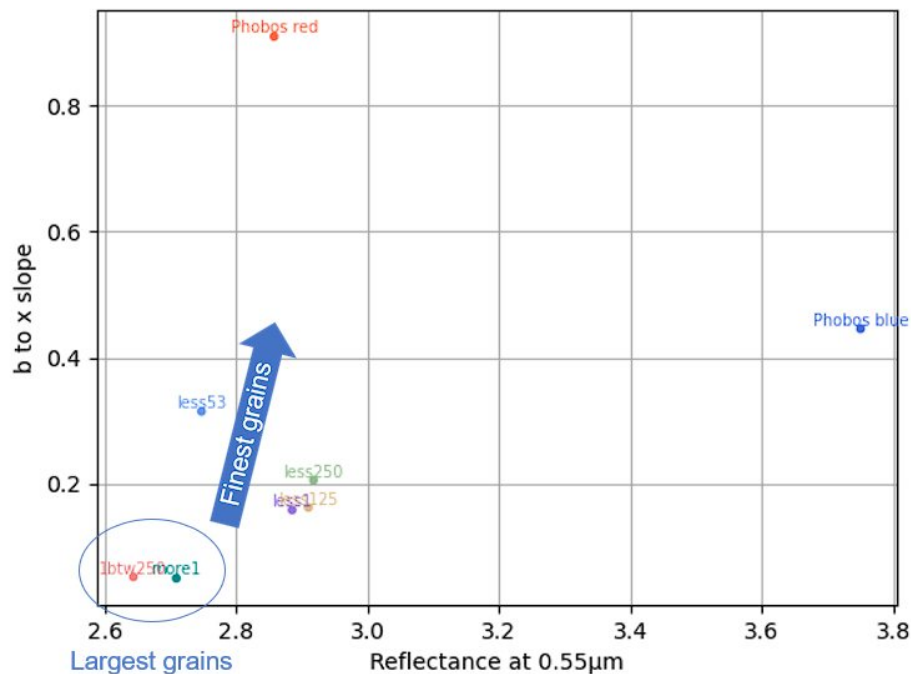
Figure 9 - b to x slope as a function to reflectance at 0.55 \mu\text{m} . Each grain size and CRISM data have been named. Smallest grains present a higher b to x slope than larger ones.
